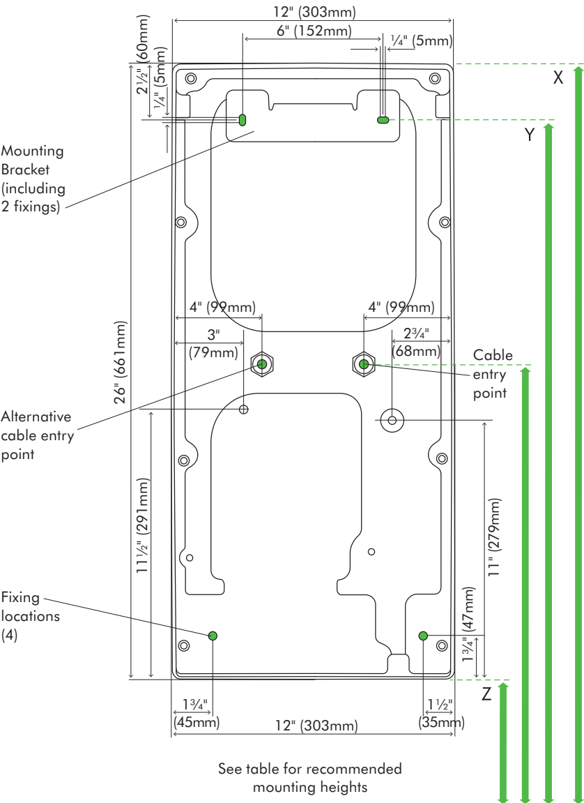
REAR ELEVATION
